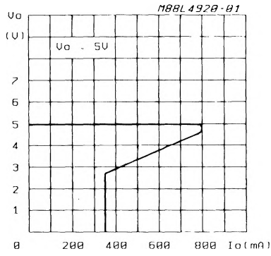
Figure 2 : Foldback Current Limiting.
