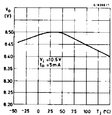
Figure 7. Output Voltage vs. Temperature (L4940V85).
