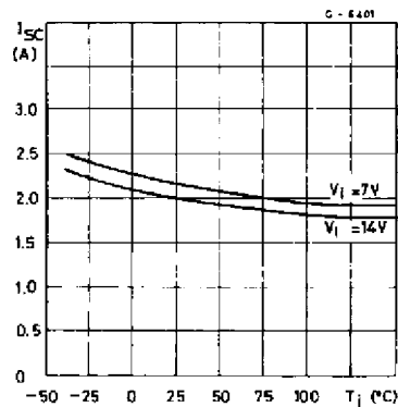
Figure 13. Short-circuit Current vs. Temperature (L4940V5).
