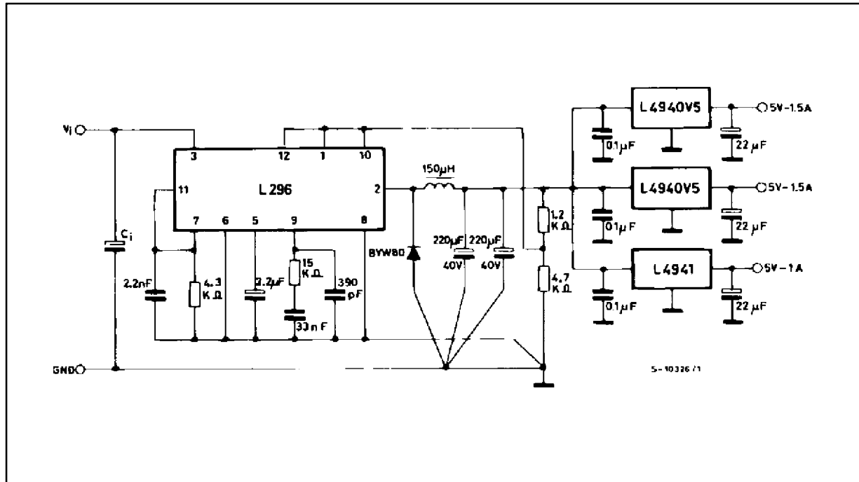
Figure 26. Distributed Supply with On-card L4940 and L4941 Low-drop Regulators.
