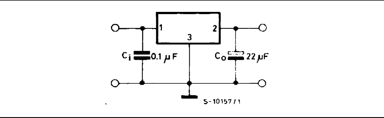
Figure 1. - DC Parameters.
