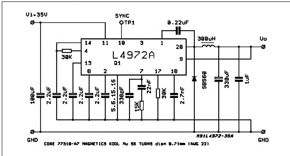
Figure 39 : 2A – 5.1V Low Cost Application Circuit.
