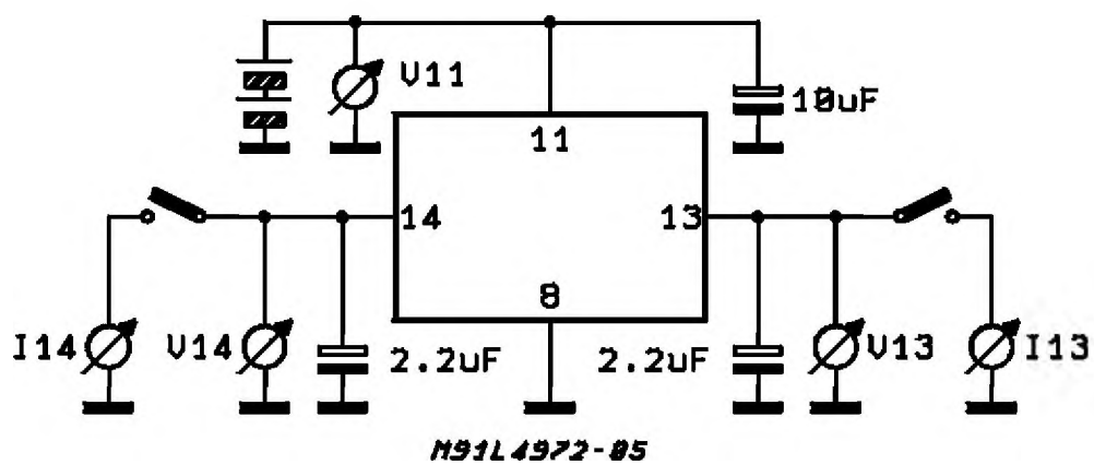
Figure 7 : DC Test Circuits.
