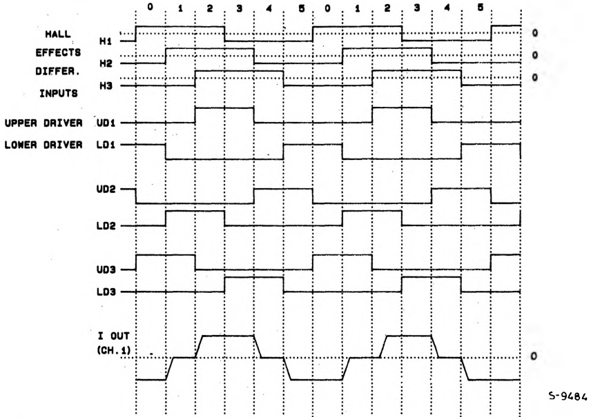
Fig. 2 - Timing diagram
