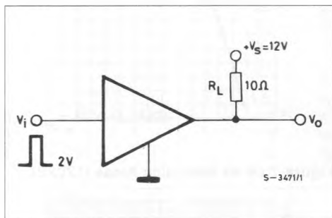
Figure 2 : t_{on} and t_{off} Test Circuit.
