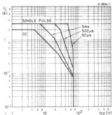
Figure 7 : Safe Operating Areas (L702B).
