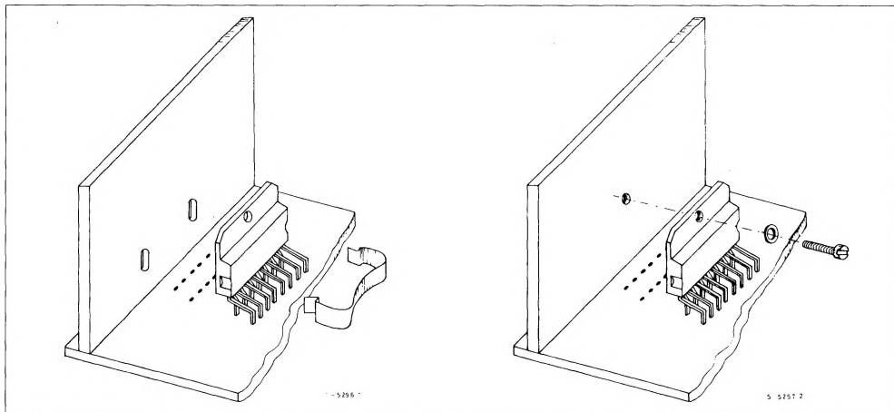
Figure 6 : Mounting Example.
