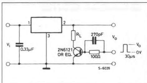
Figure 2 : Load Regulation.
