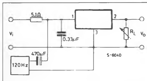
Figure 3 : Ripple Rejection.
