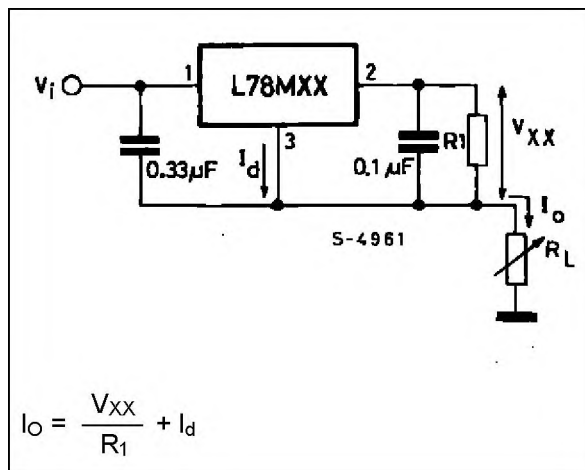
Figure 14 : Constant Current Regulator.
