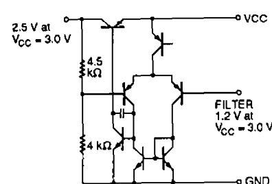
Figure 3. Preamplifier reference
