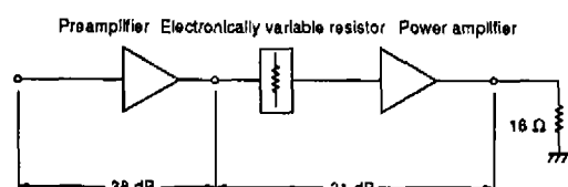
Figure 5. Preamplifier gain
