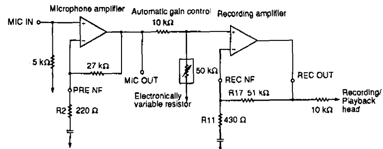
Figure 8. Microphone amplifier
