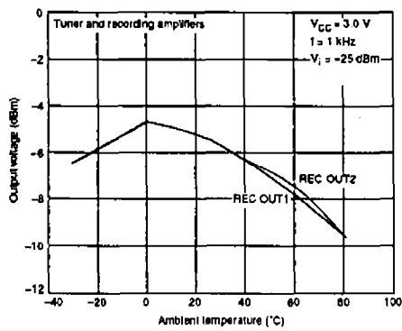
Output voltage vs. ambient temperature
