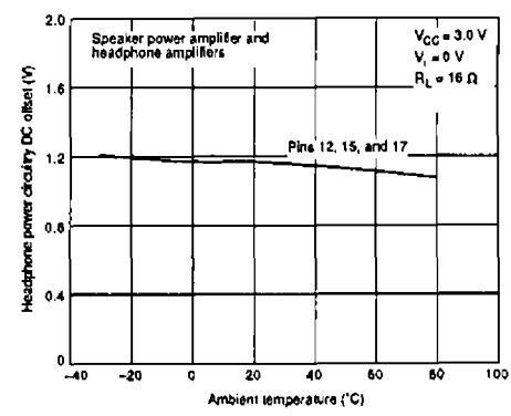
Amplifier DC offset vs. ambient temperature (7)
