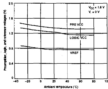
VREF, preamplifier and logic reference voltages vs. ambient temperature (1)
