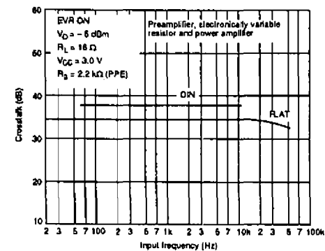
Crosstalk between channels vs. frequency
