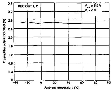
DC offset vs. ambient temperature
