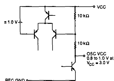
Figure 2. Oscillator supply
