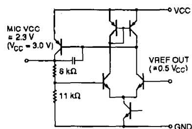
Figure 1. Microphone supply
