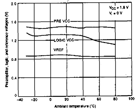
VREF, preamplifier and logic reference voltages vs. ambient temperature (2)
