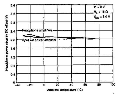
Amplifier DC offset vs. ambient temperature (8)
