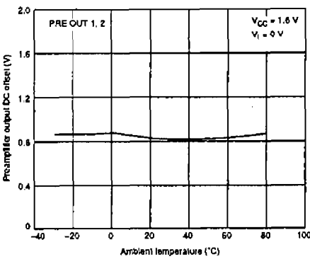
Output DC offset vs. ambient temperature (1)
