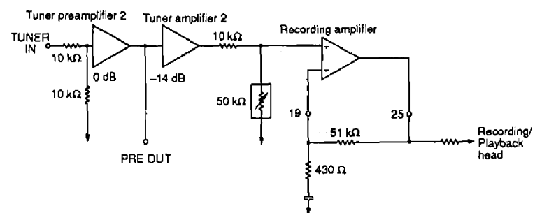
Figure 9. Tuner amplifier
