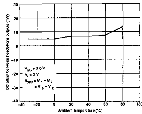
DC offset between headphone outputs vs. ambient temperature (4)
