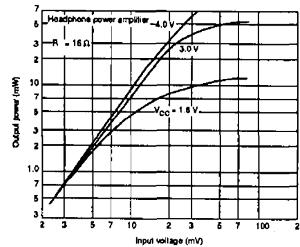
Headphone and common amplifier
