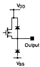
Figure 27. P-channel output option
