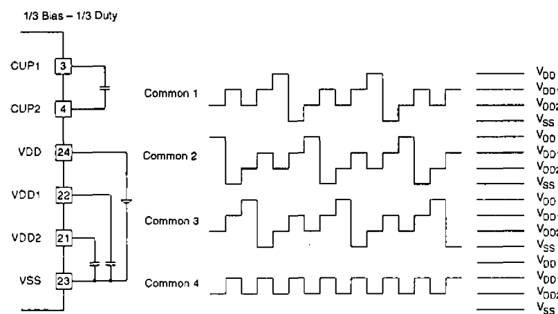
Figure 34. 1/3 bias, 1/3 duty
