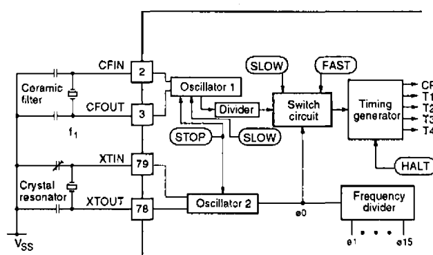
Figure 10. Ceramic filter and crystal resonators
