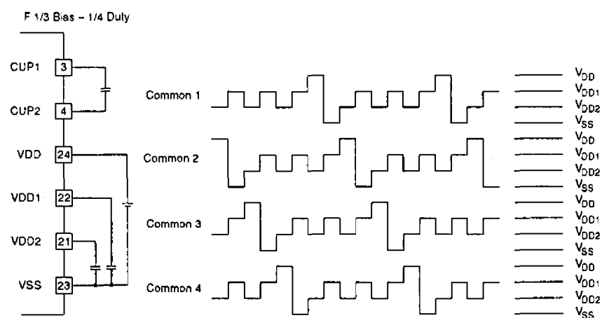
Figure 35. 1/3 bias, 1/4 duty
