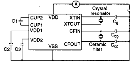
Figure 5. Supply current measurement 1
