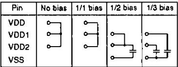
Figure 1. Supply connections
