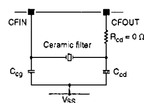
Figure 37. Ceramic filter resonator circuit
