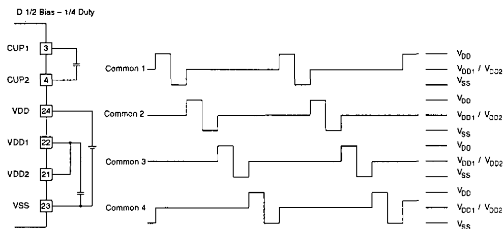
Figure 33. 1/2 bias, 1/4 duty
