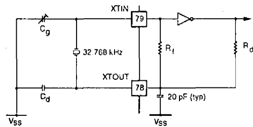
Figure 15. 32 kHz crystal
