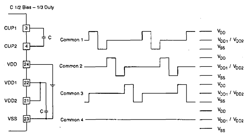
Figure 32. 1/2 bias, 1/3 duty
