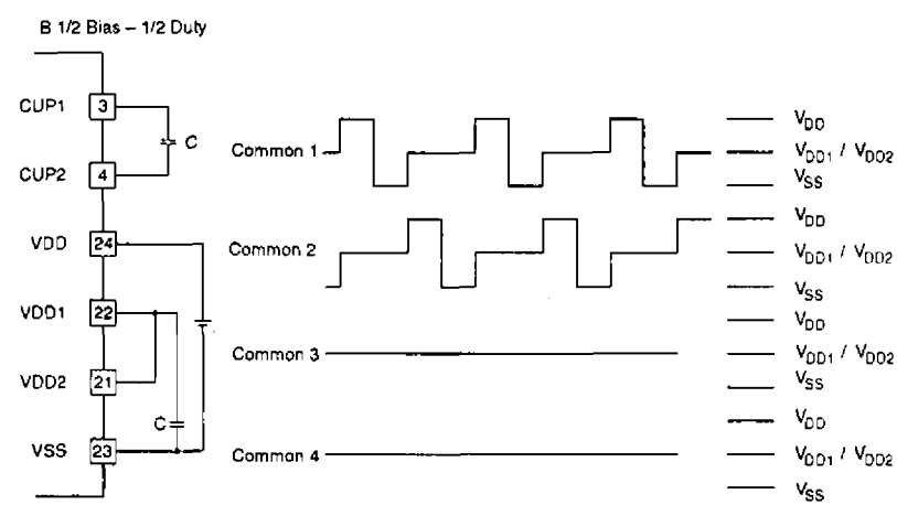
Figure 31. 1/2 bias, 1/2 duty
