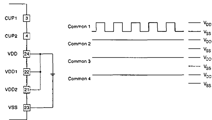
Figure 30. 1/1 bias, 1/1 duty
