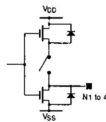
Figure 22. Port N output options
