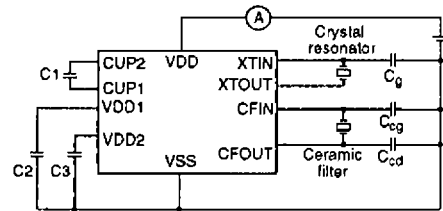
Figure 6. Supply current measurement 2
