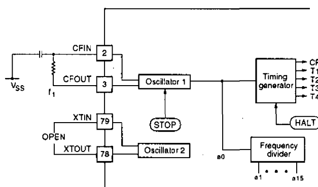
Figure 11. RC oscillator
