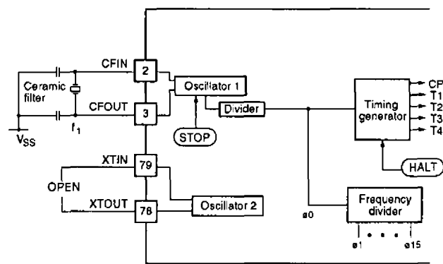
Figure 12. Ceramic filter resonator
