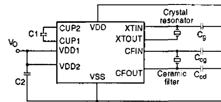
Figure 3. Output voltage measurement 1
