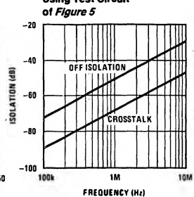
Crosstalk and "OFF" Isolation vs Frequency Using Test Circuit of Figure 5
