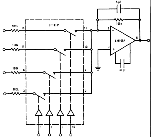
Multiplexer/Mixer
