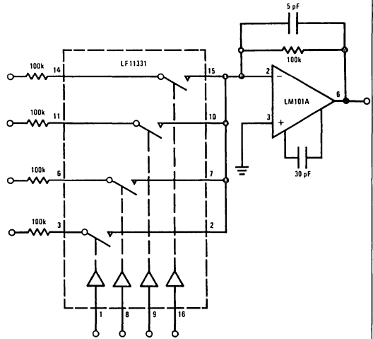
Multiplexer/Mixer
