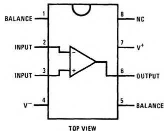
Dual-In-Line Package
