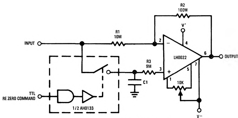
Re-Zeroing Amplifier
