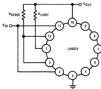
FIGURE 2. Current Limit Programmng
