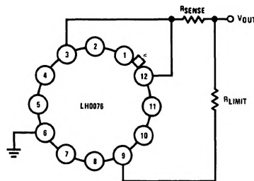
FIGURE 2. Current Limit Programming
