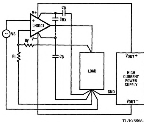
FIGURE 1. Single-Point Grounding
