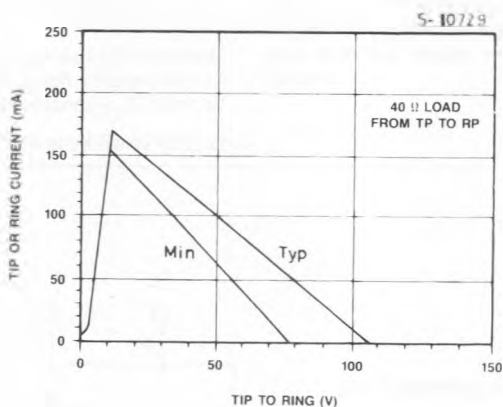
Figure 8 : Current Limiting Characteristics.
