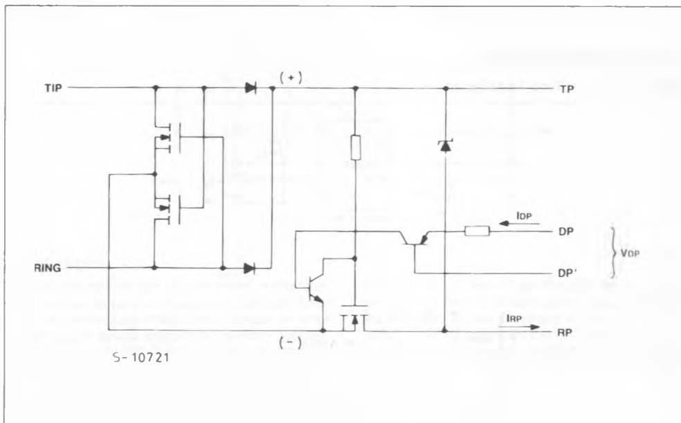
Figure 2 : Simplified Schematic Illustrating Characteristic Symbolology.
