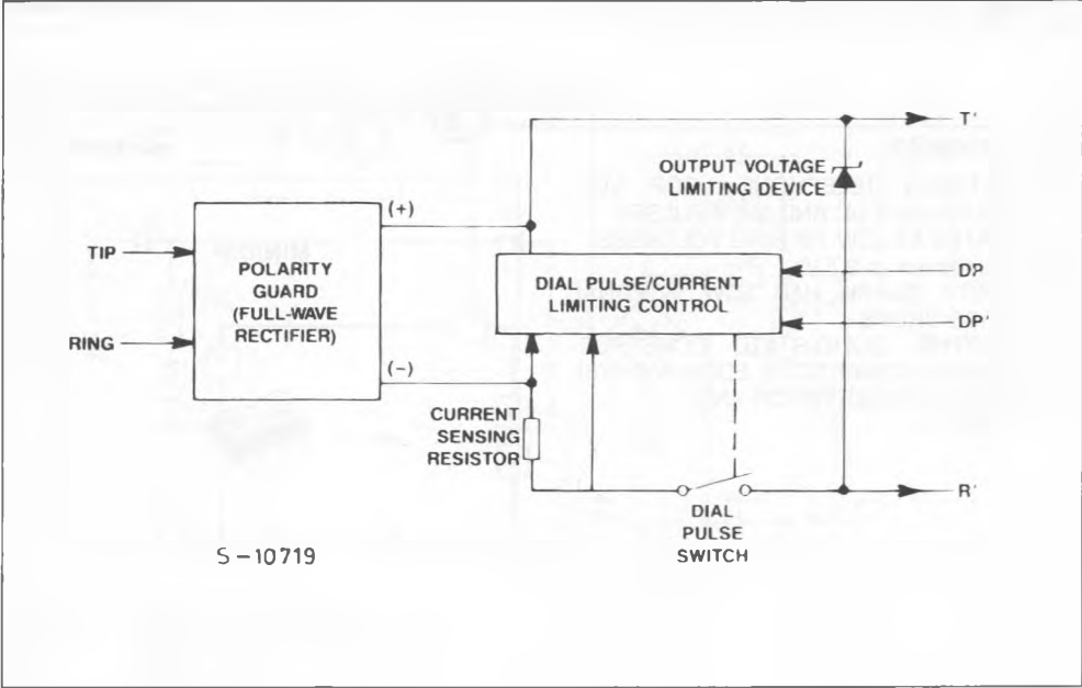
Figure 1 : Functional Diagram.
