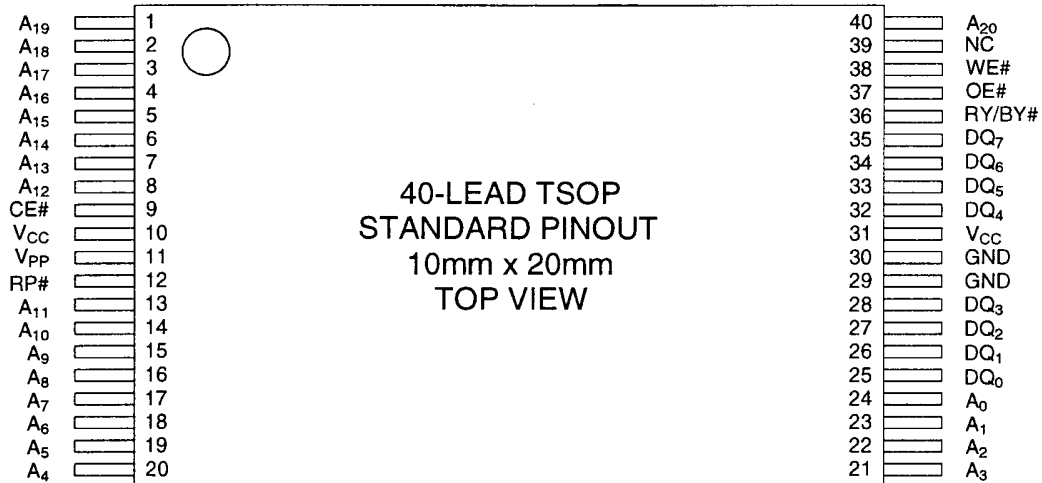
Figure 2. TSOP 40-Lead Pinout
