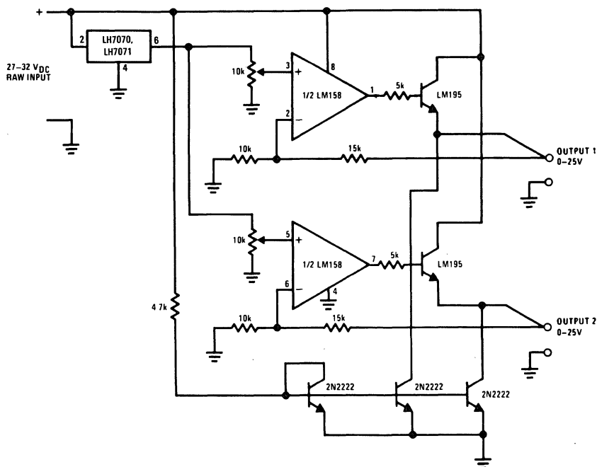
Dual Output Bench Power Supply
