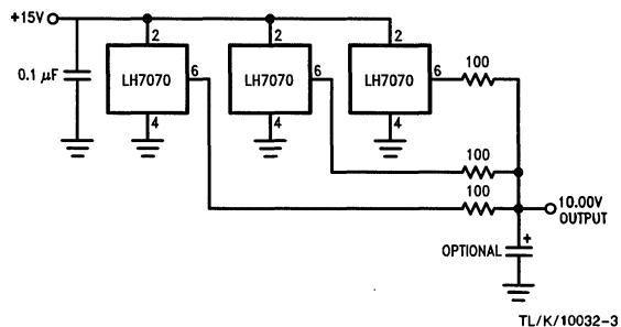
Statistical Voltage Standard
