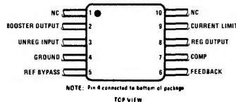
Flat Package
