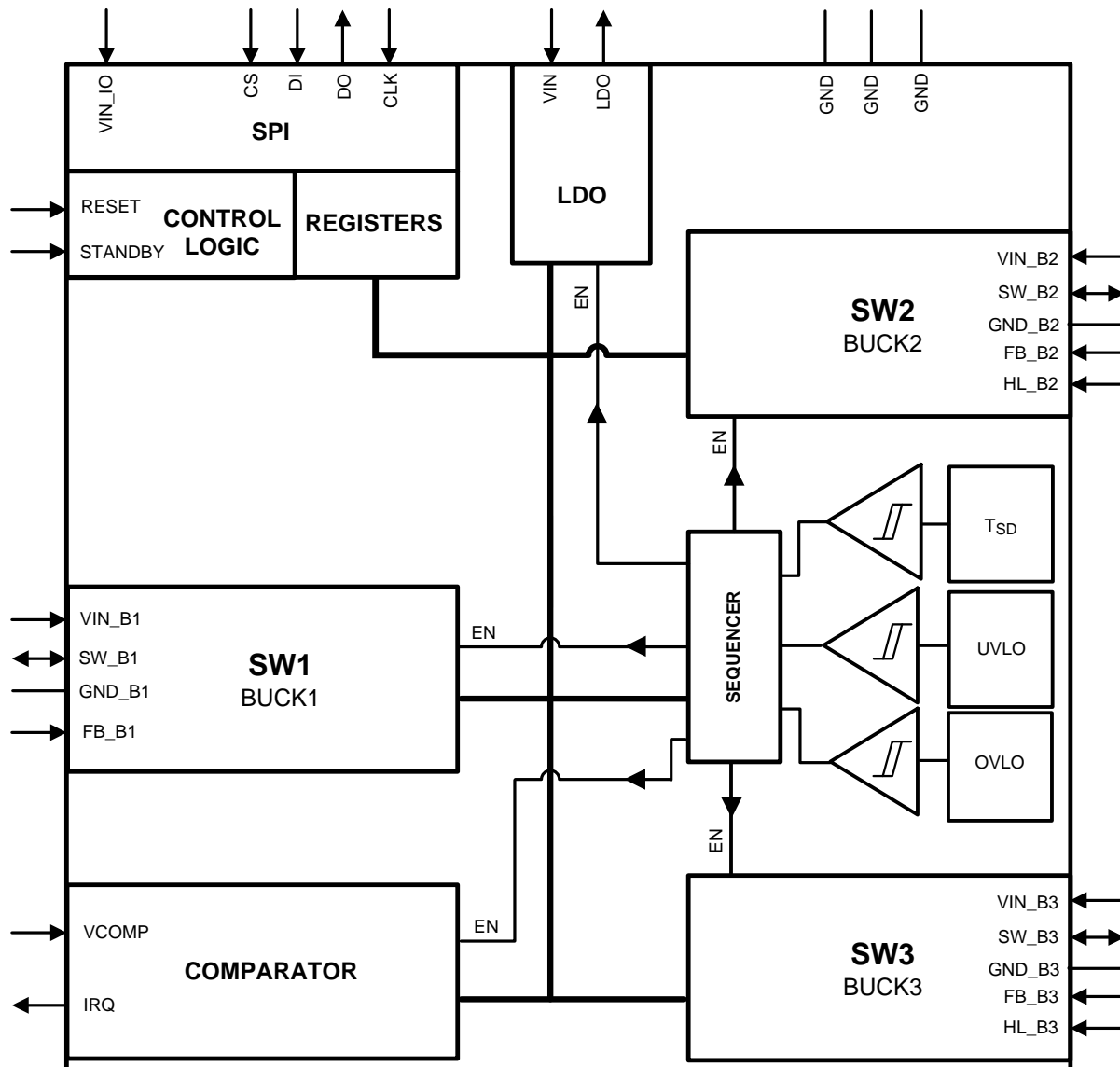
Figure 21. Internal Block Diagram of the LM10506 PMIC
