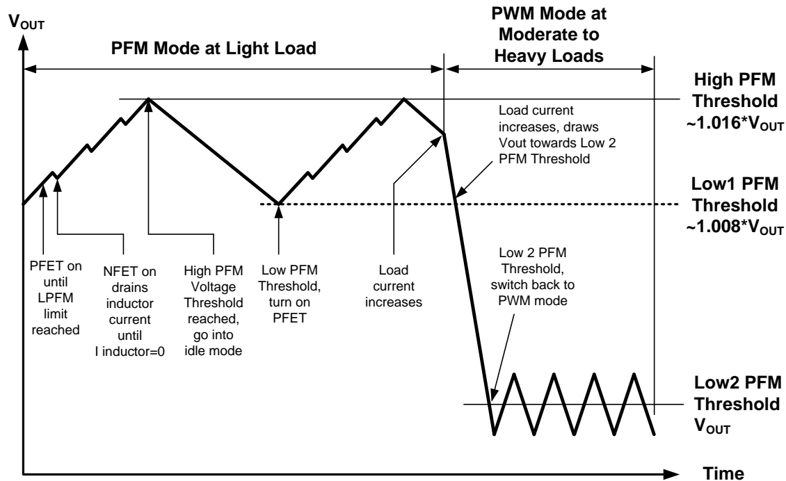
Figure 25. PFM vs PWM Operation
