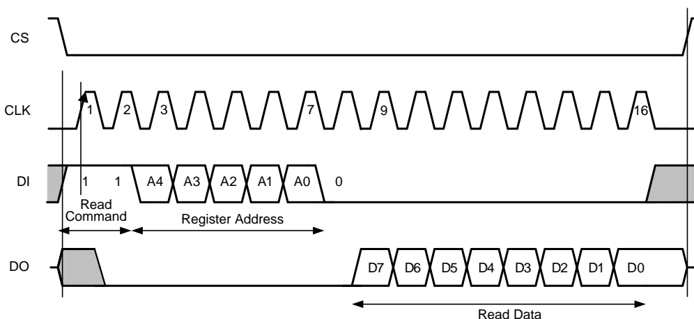
Figure 23. SPI Interface Read
