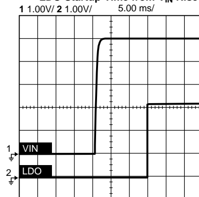
LDO Startup Time from V_{IN} Rise
