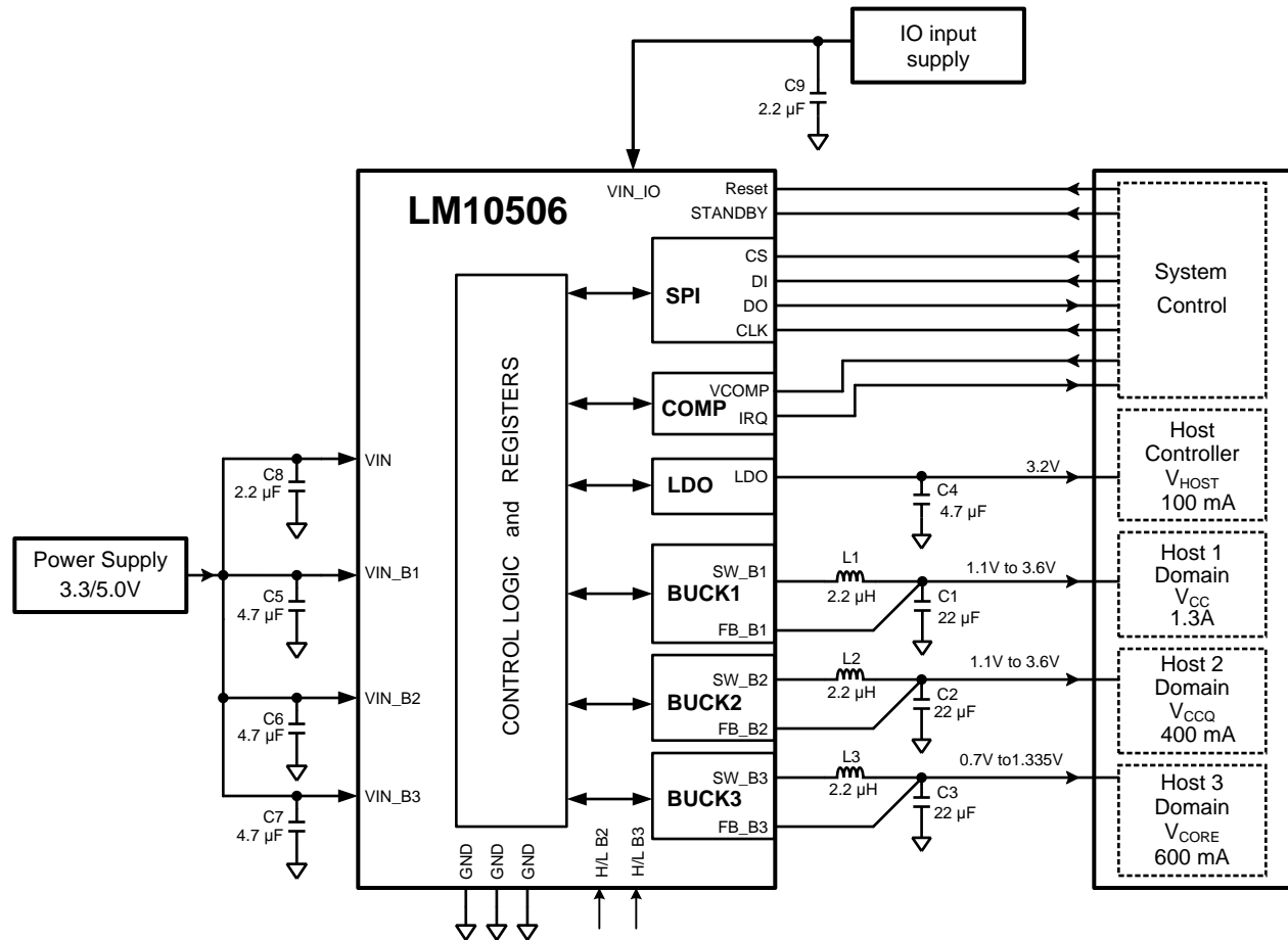
Figure 1. Typical Application Diagram
