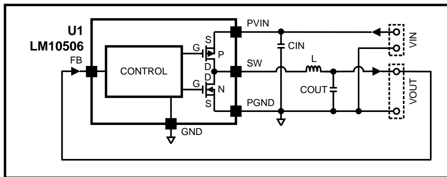
Figure 24. Buck Functional Diagram
