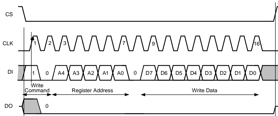
Figure 22. SPI Interface Write
