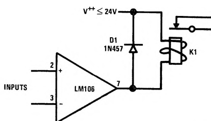
Relay Driver
