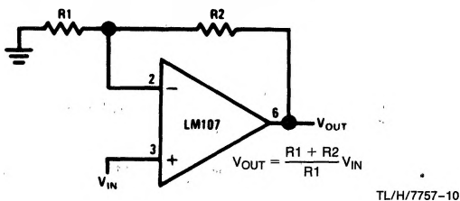
Non-Inverting Amplifier
