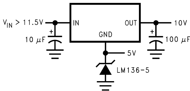
Figure 28. Regulator with Reference
