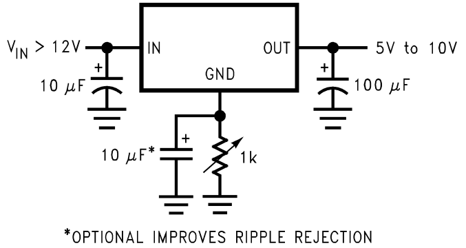
Figure 27. Adjustable Fixed Regulator
