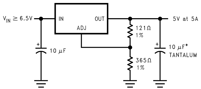
Figure 23. Adjustable @ 5V
