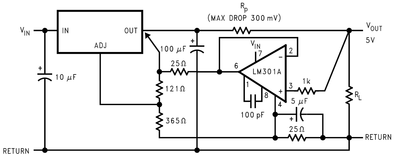
Figure 34. Remote Sensing
