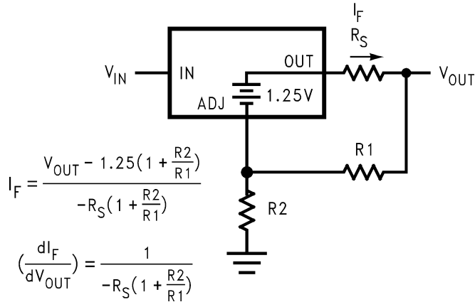
Figure 26. Battery Charger
