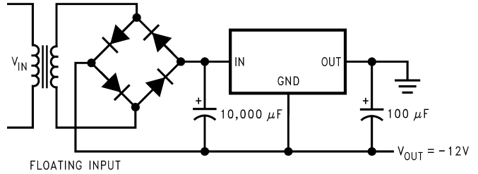
Figure 33. Generating Negative Supply voltage
