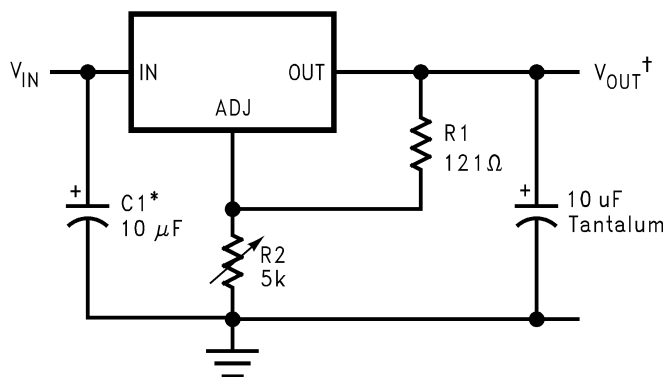
Figure 22. 5V to 3.3V, 5A Regulator
