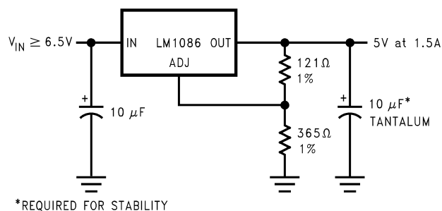
Figure 26. Adjustable @ 5V
