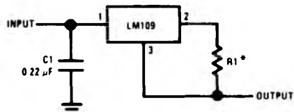
Current Regulator
