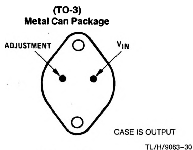
Bottom View Steel Package Order Number LM117K STEEL or LM317K STEEL See NS Package Number K02A Order Number LM117K/883 See NS Package Number K02C
