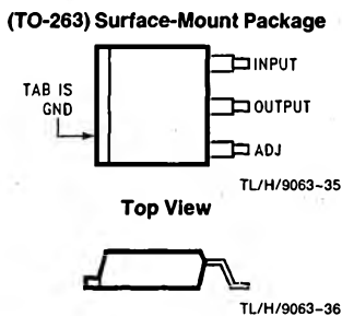
Top View Side View Order Number LM317S See NS Package Number TS3B
