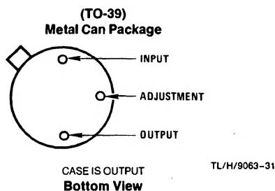
Bottom View Order Number LM117H, LM117H/883, LM317AH or LM317H See NS Package Number H03A
