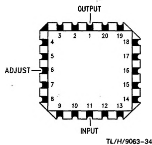
Top View Order Number LM117E/883 See NS Package Number E20A
