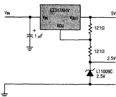
Regulator with Reference
