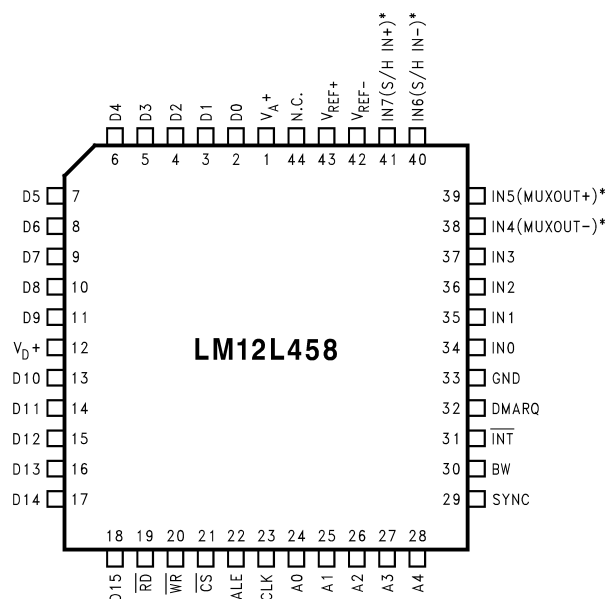
Figure 1. Connection Diagram
