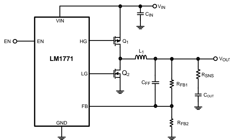
Figure 21. Example Circuit Schematic
