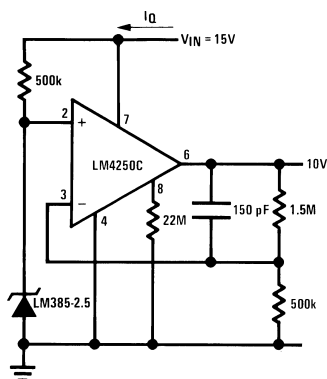
Figure 18. Micropower 10V Reference
