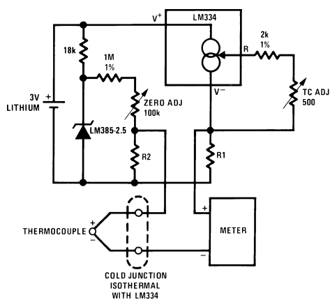
Figure 20. 0°F–50°F Thermomemter
