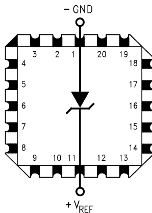
Figure 4. LCCC Leadless Chip Carrier See Package Number NAJ0020A
