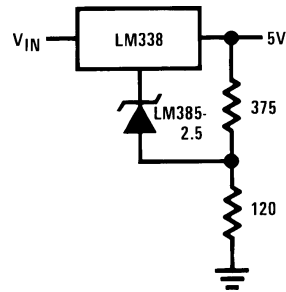
Figure 22. Improving Regulation of Adjustable Regulators
