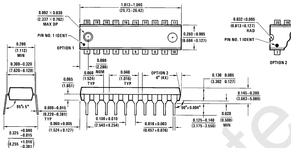
Molded Dual-in-Line Package (N) Order Number LM1865N NS Package Number N20A
