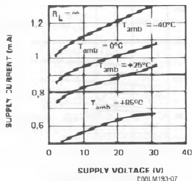
SUPPLY CURRENT
