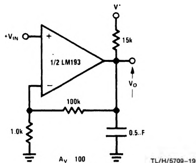
Low Frequency Op Amp
