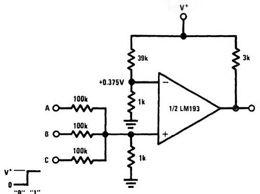
AND Gate
