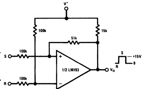
Bi-Stable Multivibrator
