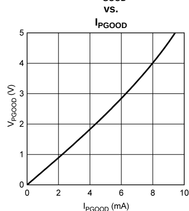
P_{GOOD}
