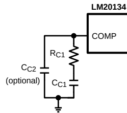
Figure 6. Compensation Network for LM20134
