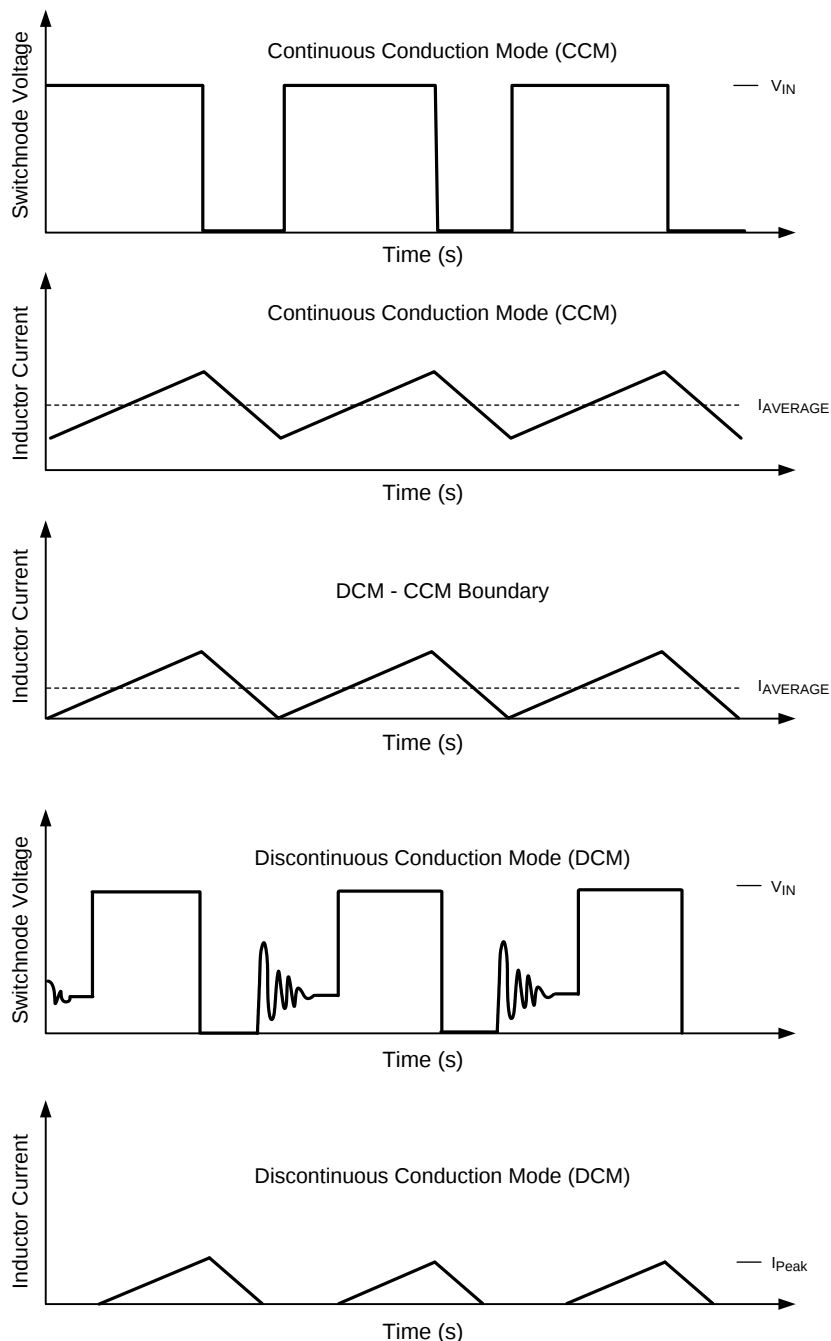
Figure 2. Modes of Operation for LM20134
