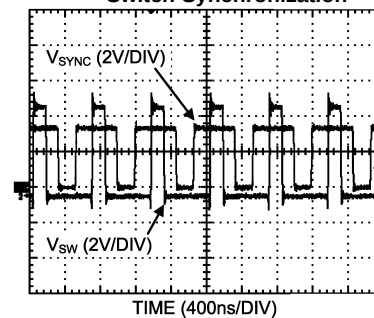
Switch Synchronization
