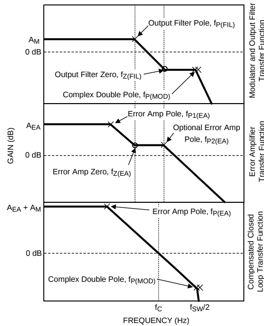
Figure 5. LM20134 Loop Compensation
