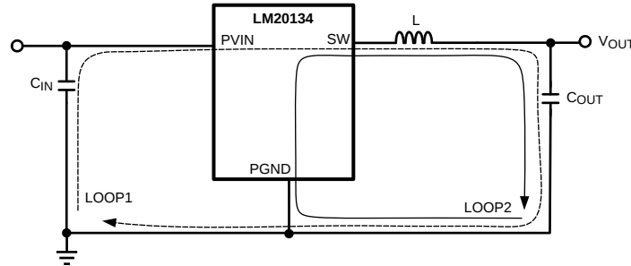
Figure 11. Schematic of LM20134 Highlighting Layout Sensitive Nodes
