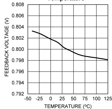
Feedback Pin Voltage vs. Temperature
