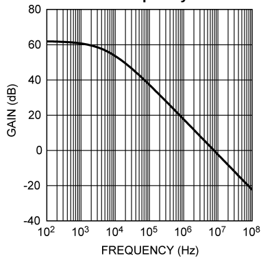
Error Amplifier Gain vs. Frequency
