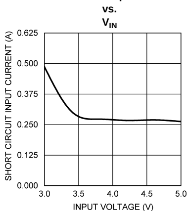
Short Circuit Input Current
