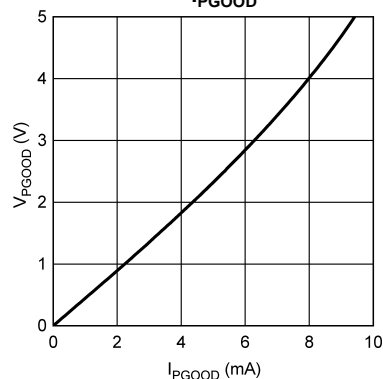
P_{GOOD} vs. I_{PGOOD}
