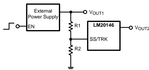
Figure 9. Tracking an External Supply
