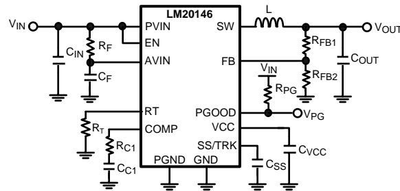
Figure 4. Typical Application Circuit
