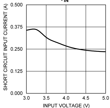
Short Circuit Input Current vs. V_{IN}
