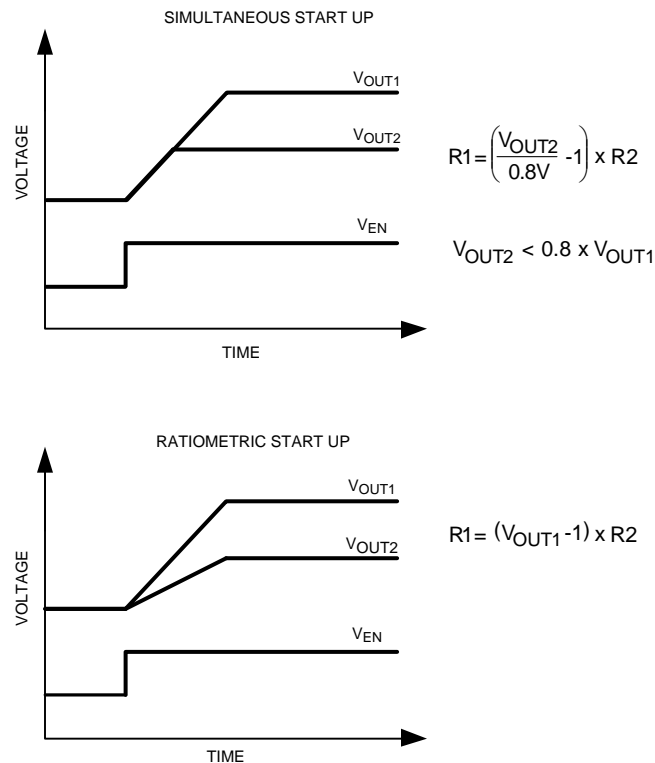
Figure 10. Common Start Up Sequences
