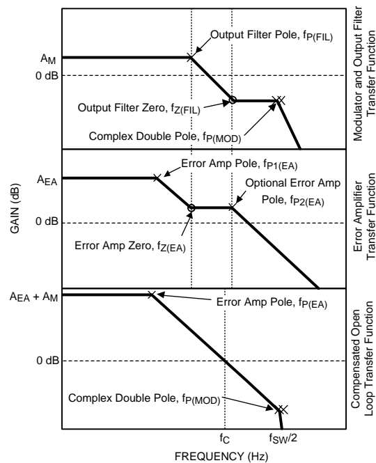
Figure 6. LM20146 Loop Compensation
