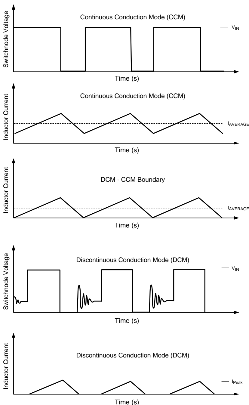
Figure 3. Modes of Operation for LM20146
