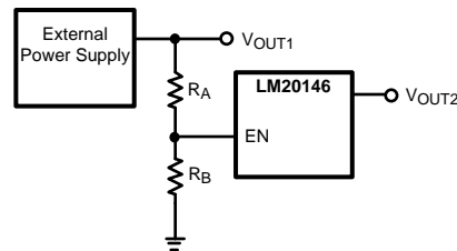
Figure 8. Sequencing LM20146 with Precision Enable
