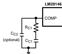
Figure 7. Compensation Network for LM20146
