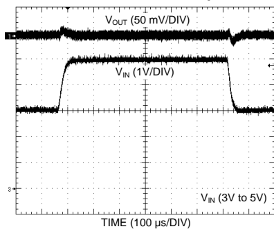
Start-Up (Tracking)
