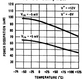
Power Consumption
