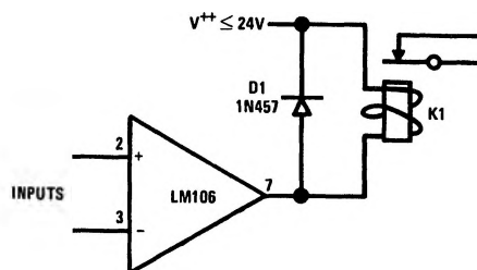
Relay Driver
