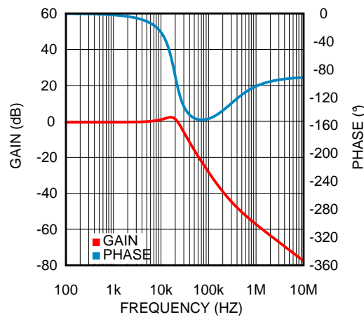
Figure 34. Power Train Bode Plot
