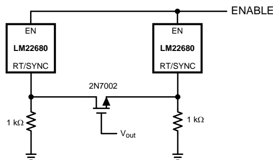
Figure 19. Self Synchronizing Setup
