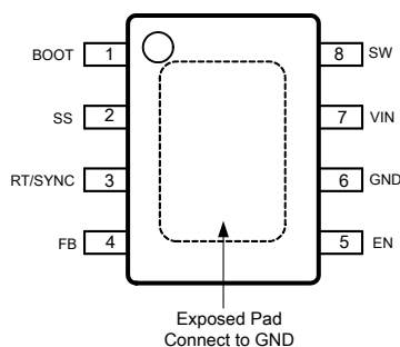
Figure 1. Connection Diagram Package Number MRA08B
