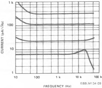
CURRENT NOISE
