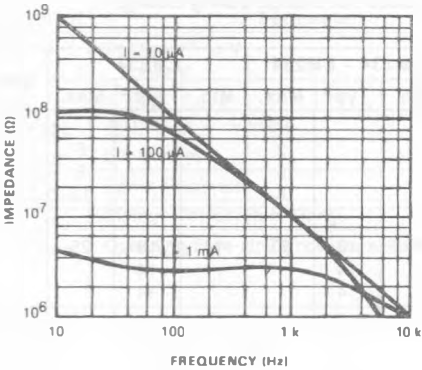
OUTPUT IMPEDANCE
