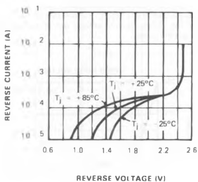
REVERSE CHARACTERISTICS
