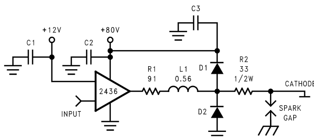
Figure 10. One Channel of the LM2436 with the Recommended Application Circuit
