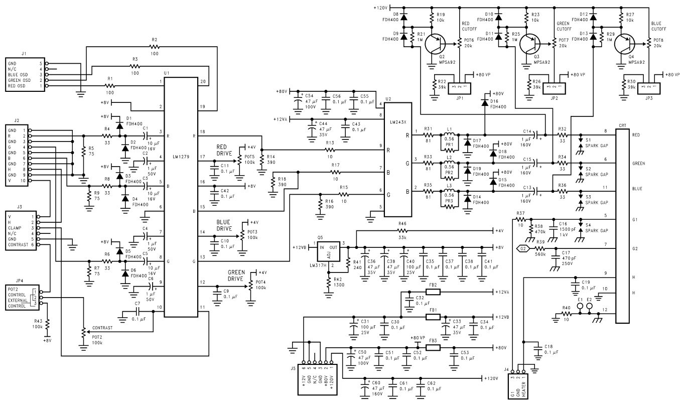
Figure 12. LM1279/243X Demonstration Board Schematic
