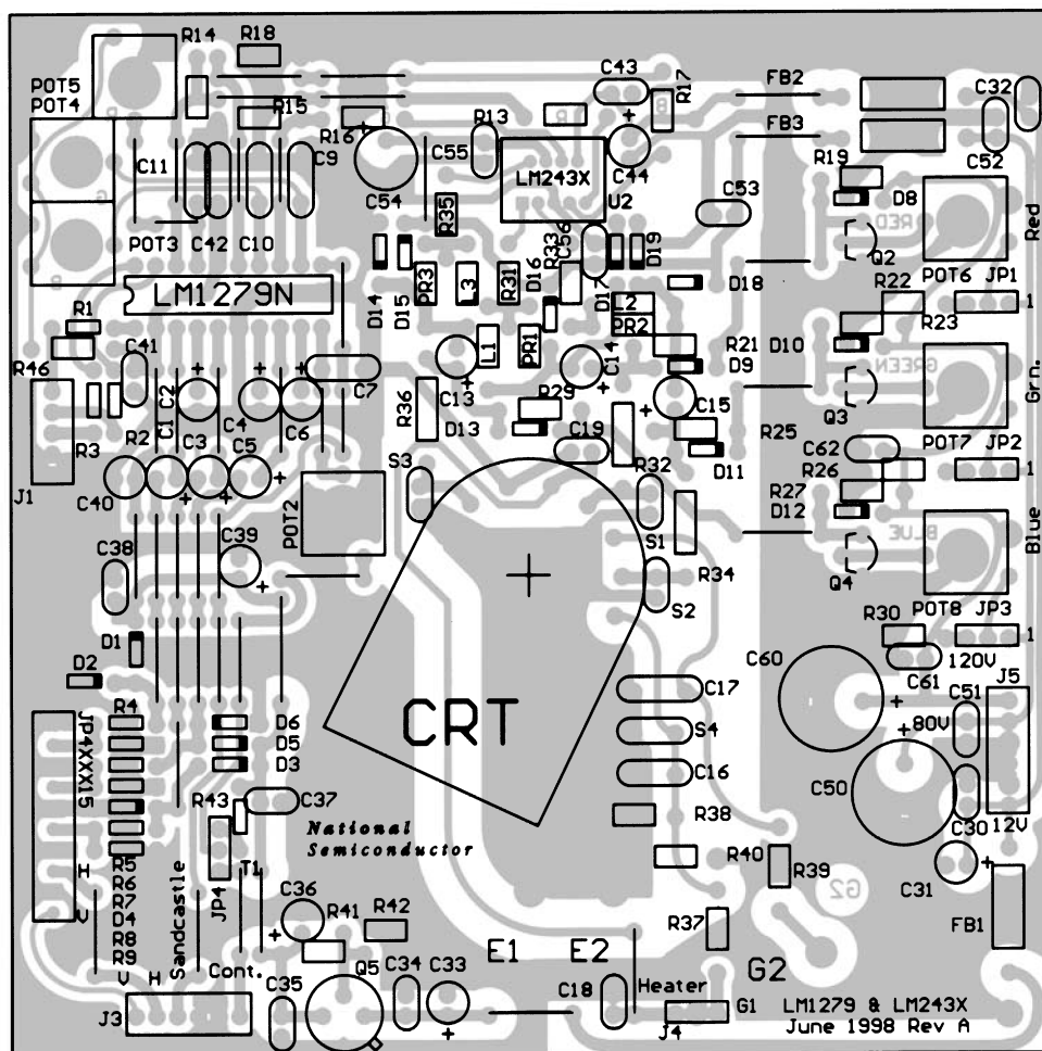
Figure 13. LM1279/243X Demo Board Layout
