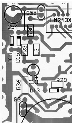
Figure 14. Trace Routing and Component Placement for Blue Channel Output
