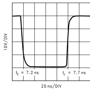
Figure 6. LM2436 Pulse Response
