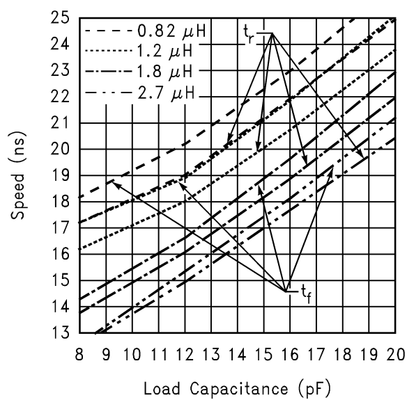
FIGURE 8. Speed vs Load Capacitance for Various Inductances
