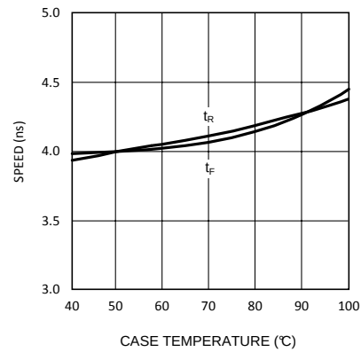
Figure 5. Speed vs Temp.
