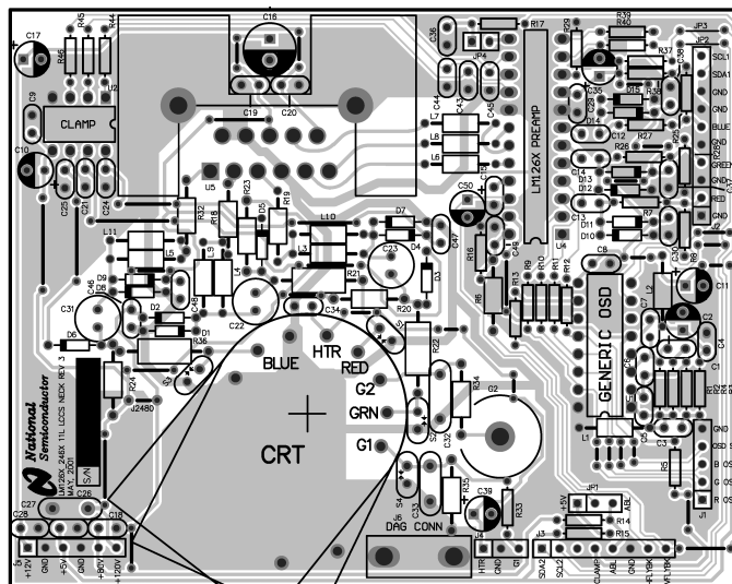
Figure 13. NSC Demonstration Board Layout
