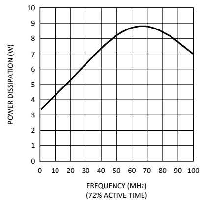
Figure 7. Power Dissipation vs Frequency
