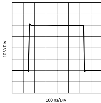
Figure 6. LM2471 Pulse Response
