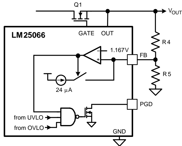
Figure 45. Programming the PGD Threshold
