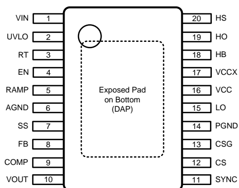
Figure 1. Top View 20-Lead HTSSOP with Exposed Pad Package Number PWP0020A
