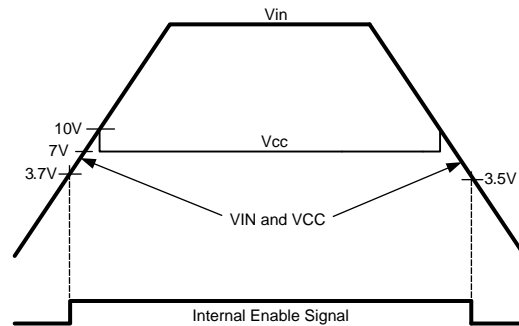
Figure 13. VIN and VCC Sequencing
