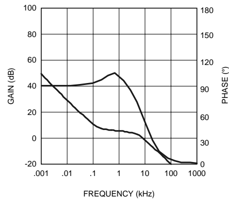
Figure 21. Error Amplifier Gain and Phase
