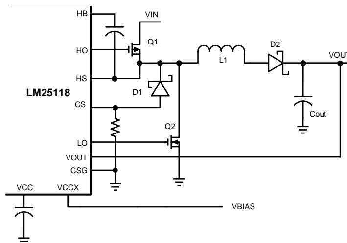
Figure 24. VCC Bias with Additional Bias Supply
