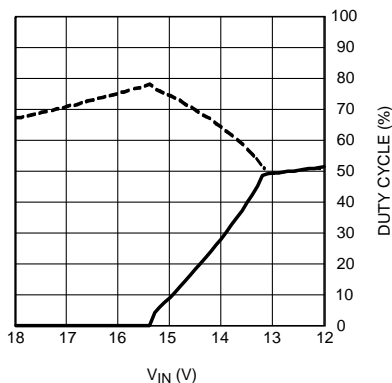
Figure 11. Mode Dependence on Duty Cycle (V OUT = 12V)
