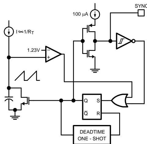
Figure 15. Simplified Oscillator and Block Diagram with Sync I/O Circuit
