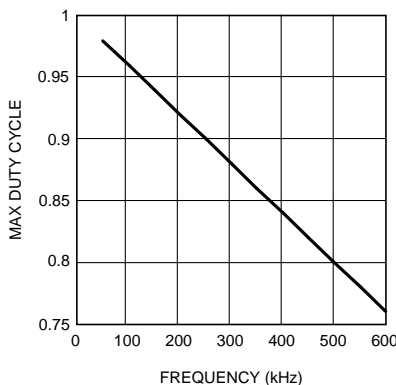
Figure 18. Maximum Duty Cycle vs Frequency
