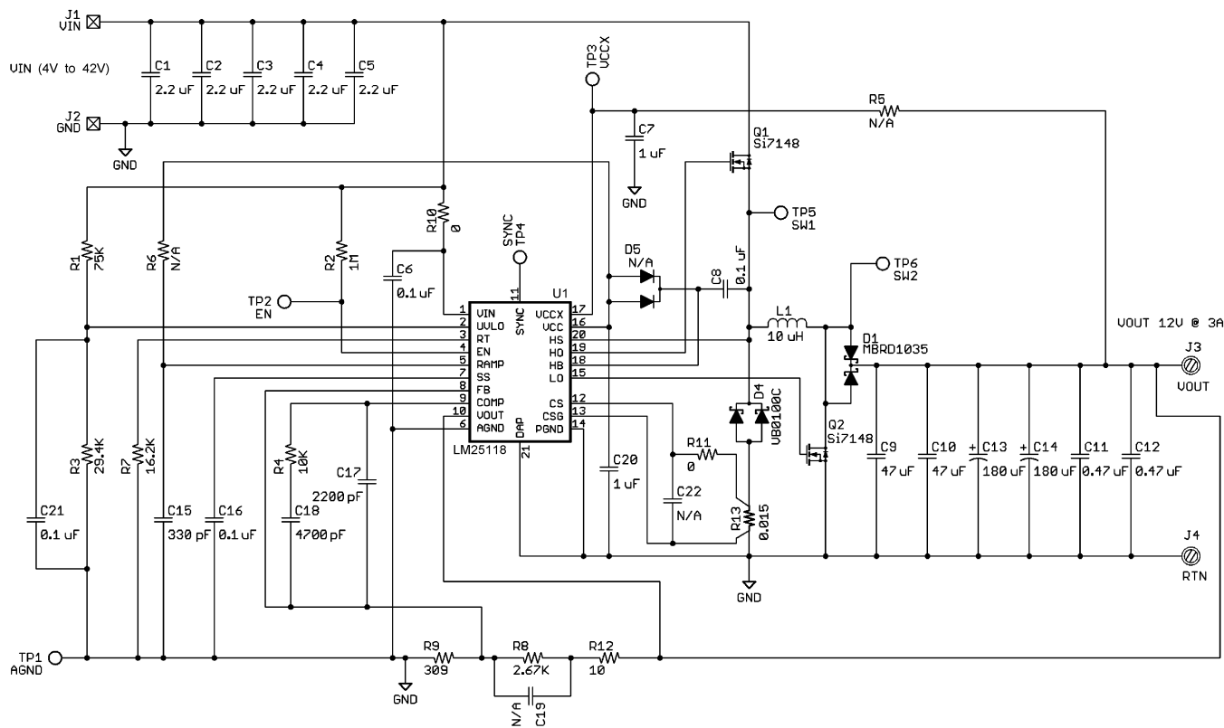
Figure 25. 12V, 3A Typical Application Schematic
