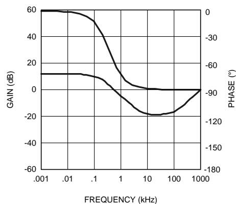
Figure 20. Modulator Gain and Phase
