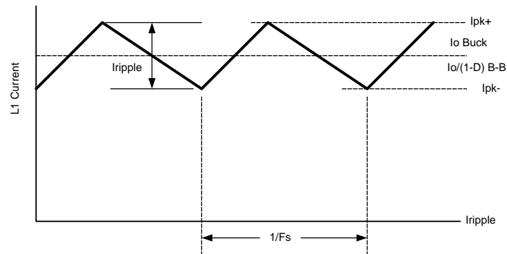
Figure 19. Inductor Current Waveform
