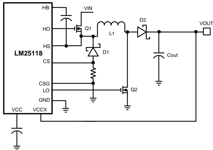
Figure 23. VCC Bias from VOUT 4V < VOUT < 15V
