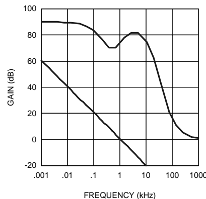
Figure 22. Overall Loop Gain and Phase
